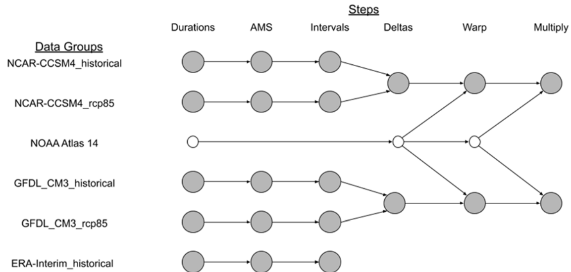
Figure 13: Schematic of data pipeline
